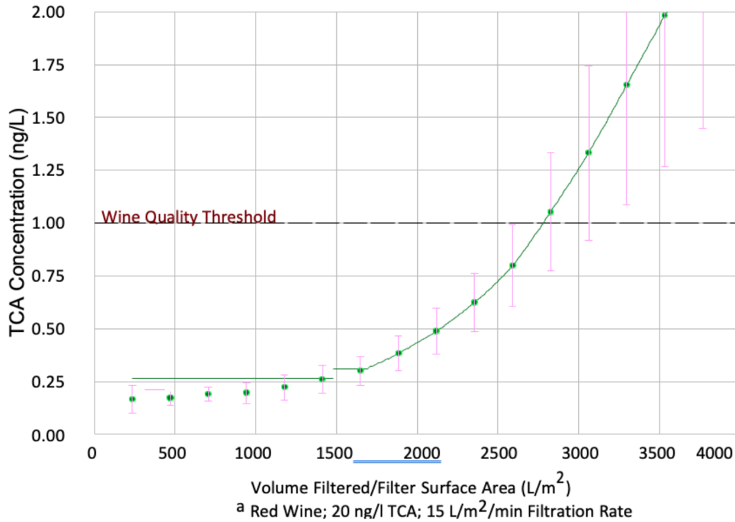
Efficacy of Depth Filtration Sheets Containing Selective Zeolite Y-Faujasite TCA Breakthrough Curve a
